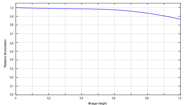
Relative illumination 像面照度比
